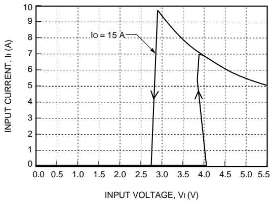
Figure 2. NH050M-L Input Characteristics, T_A = 25^\circ\text{C}
