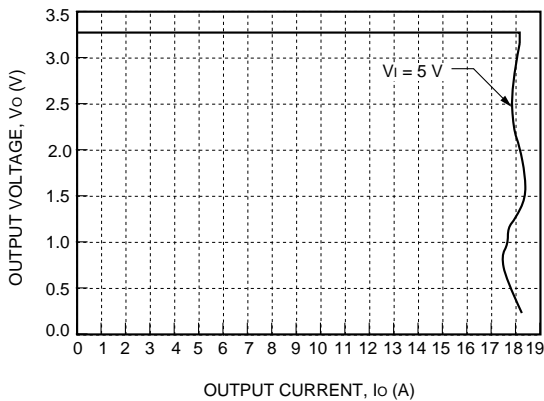
Figure 15. NH033F-L Current Limit, T_A = 25^\circ\text{C}
