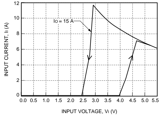
Figure 4. NH050S1R8-L Input Characteristics, T_A = 25^\circ\text{C}
