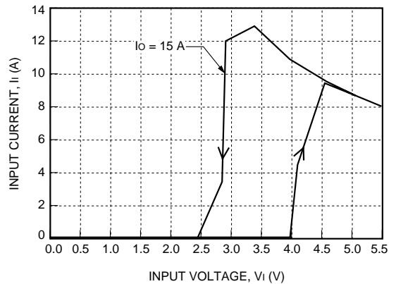
Figure 6. NH050G-L Input Characteristics, T_A = 25^\circ\text{C}
