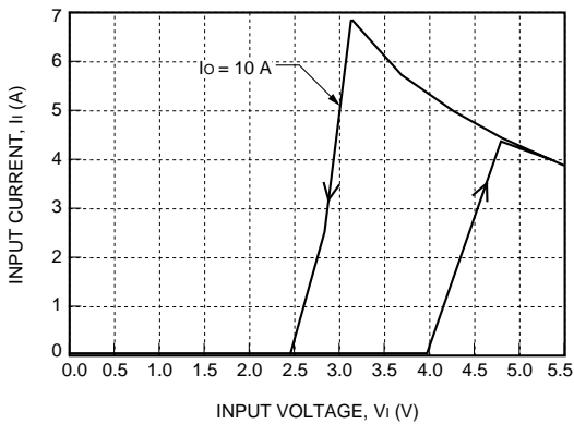
Figure 3. NH033S1R8-L Input Characteristics, T_A = 25^\circ\text{C}
