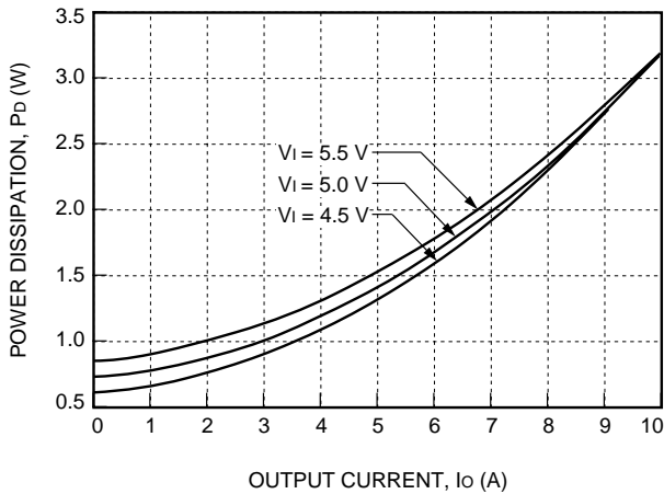
Figure 44. NH033S1R8-L Typical Power Dissipation vs. Output Current, T_A = 25\text{ }^\circ\text{C}
