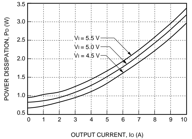
Figure 46. NH033G-L Typical Power Dissipation vs. Output Current, T_A = 25\text{ }^\circ\text{C}
