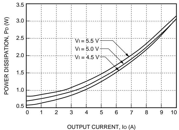
Figure 42. NH033M-L Typical Power Dissipation vs. Output Current, TA = 25 °C
