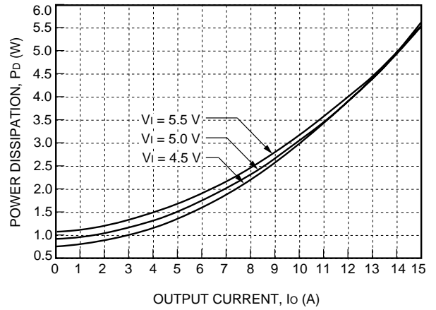
Figure 45. NH050S1R8-L Typical Power Dissipation vs. Output Current, T_A = 25\text{ }^\circ\text{C}
