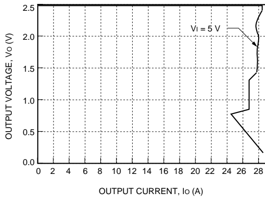
Figure 14. NH050G-L Current Limit, T_A = 25^\circ\text{C}
