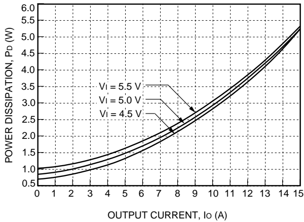
Figure 43. NH050M-L Typical Power Dissipation vs. Output Current, T_A = 25\text{ }^\circ\text{C}
