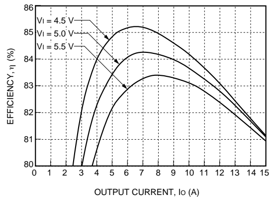
Figure 18. NH050M-L Efficiency, T_A = 25^\circ\text{C}
