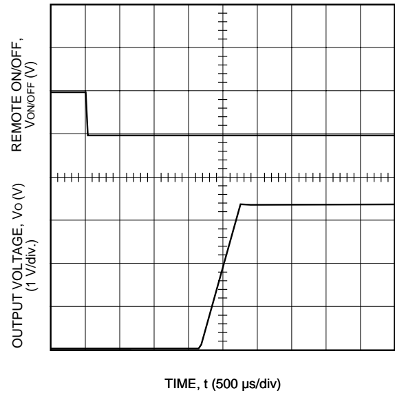
Figure 32. NH050F-L Typical Start-Up from Remote On/Off, V I = 5 V, I o = 15 A
