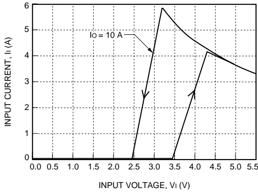
Figure 1. NH033M-L Input Characteristics, T_A = 25^\circ\text{C}
