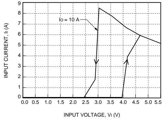
Figure 5. NH033G-L Input Characteristics, T_A = 25^\circ\text{C}
