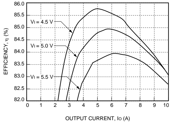
Figure 17. NH033M-L Efficiency, T_A = 25^\circ\text{C}
