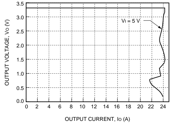
Figure 16. NH050F-L Current Limit, T_A = 25^\circ\text{C}
