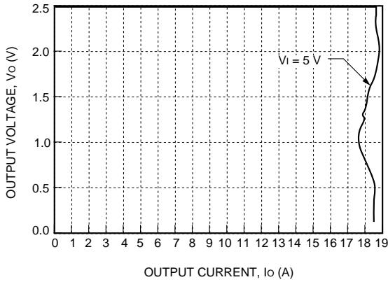
Figure 13. NH033G-L Current Limit, T_A = 25^\circ\text{C}
